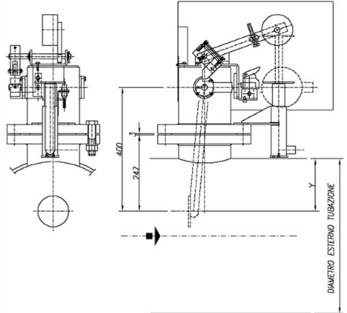
Version for electric resetting pump
